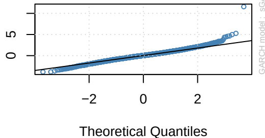
norm - QQ Plot
