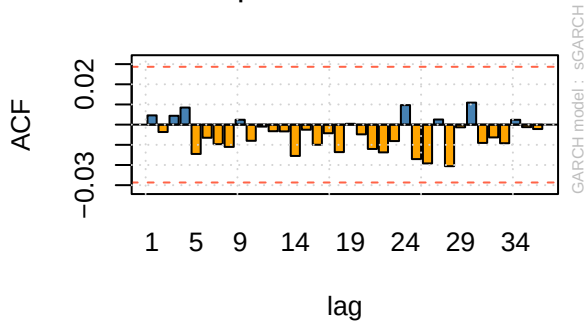
ACF of Squared Standardized Residuals
