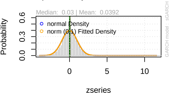
Empirical Density of Standardized Residuals
